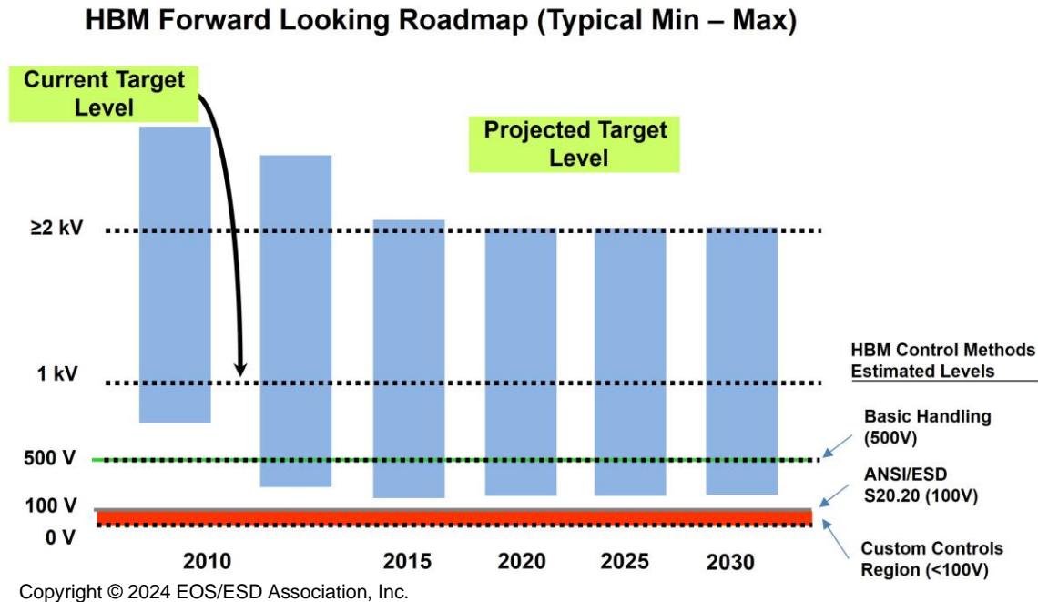
Figure 1: 2010 to 2030 Human Body Model Sensitivity Limits Projections
