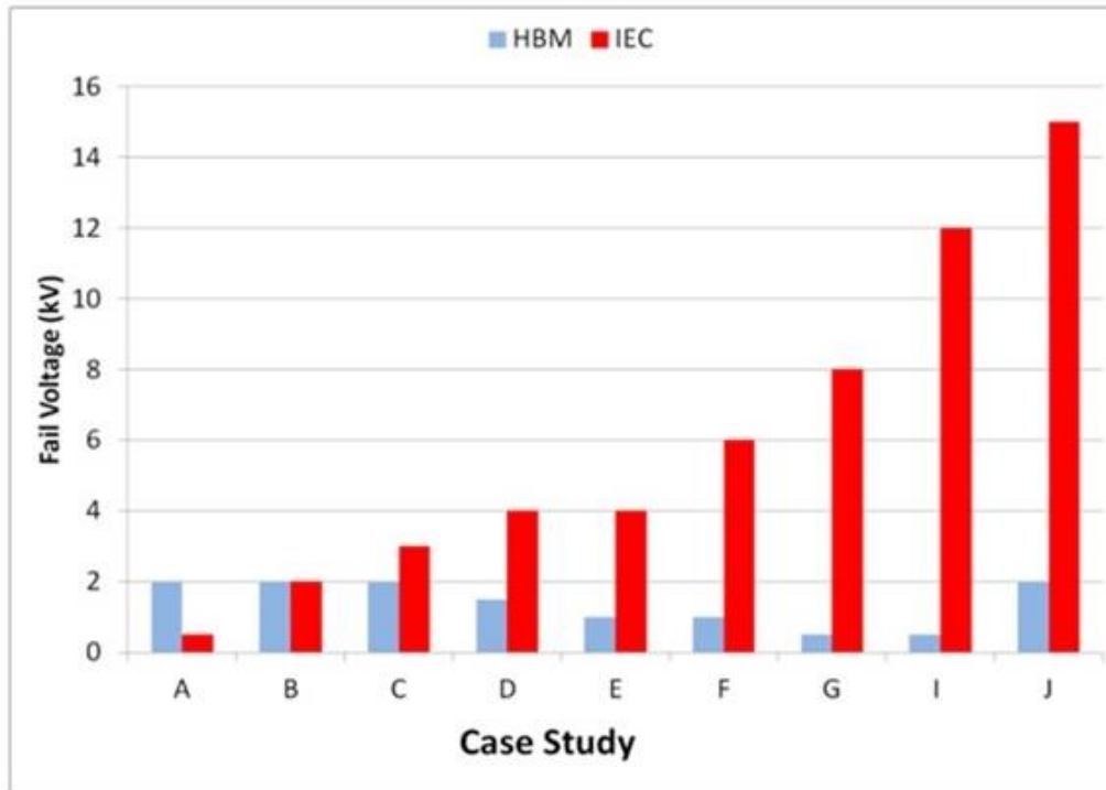
Figure 6: Comparison of IC Device Level and System Level ESD Failure Threshold of Various Systems (A-J) Showing that HBM Protection is not Related to System Level ESD Robustness
