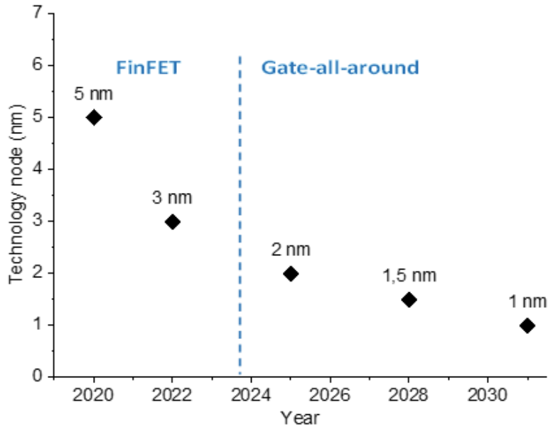
Figure 10: Roadmap for Logic Device Scaling Until 2031
