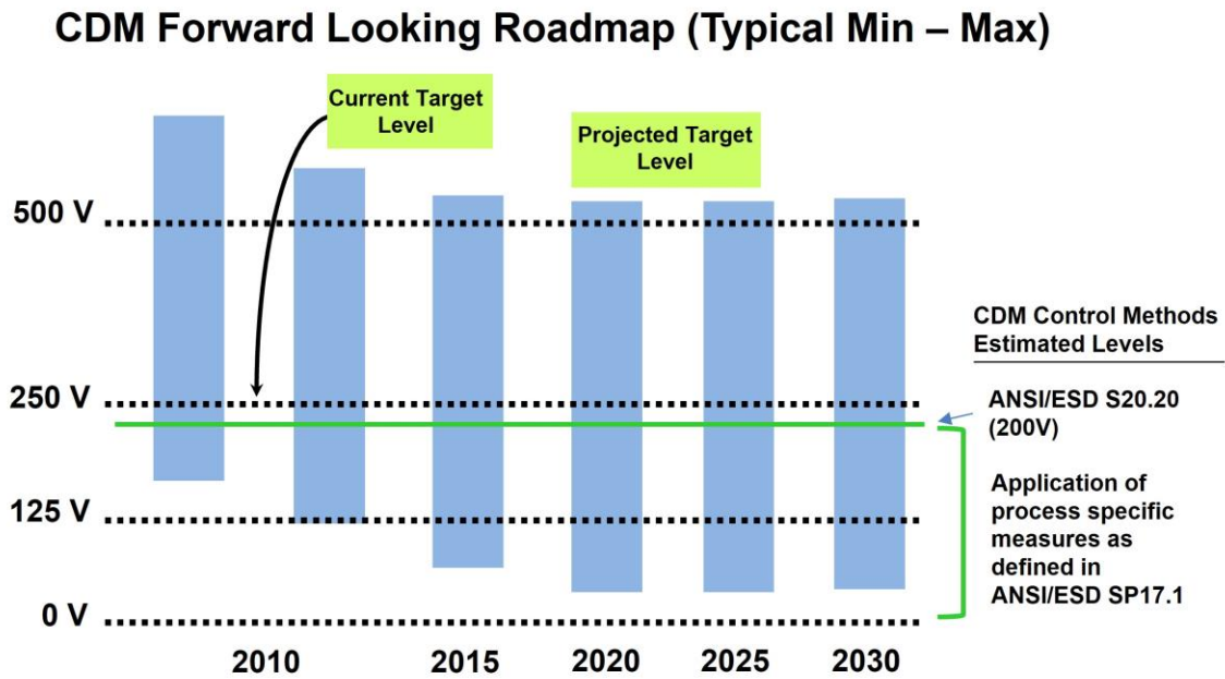
Figure 4: 2010 to 2030 Charged Device Model Sensitivity Limits Projections
