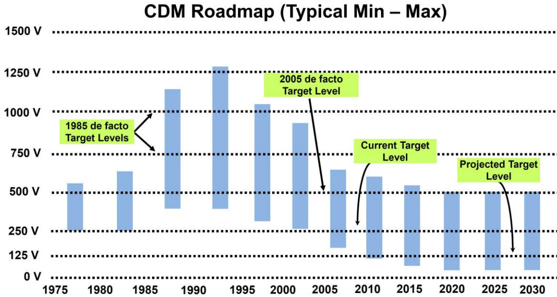
Figure 3: Overall Charged Device Model Sensitivity Limits Projections
