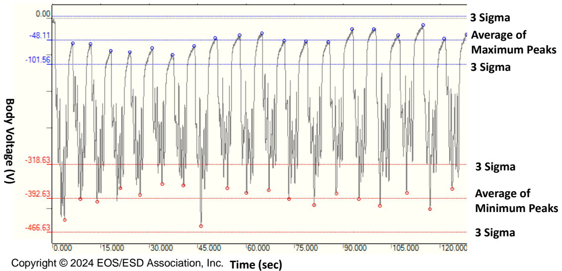
Figure 9: Determining Process Capability of a Footwear/Flooring System using ANSI/ESD STM97.2
