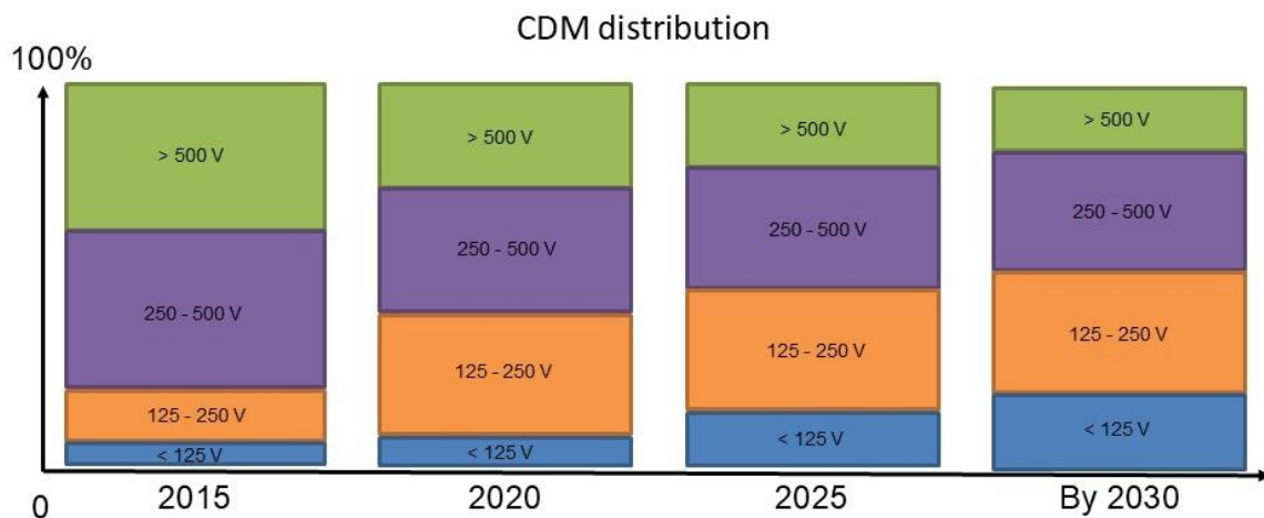
Figure 5: Forward-Looking Charged Device Model Sensitivity Distribution Groups
