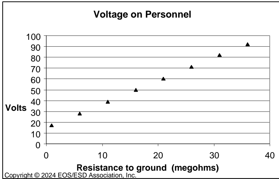
Figure 8: Relationship Between Body Voltage and Resistance to Ground [2]
