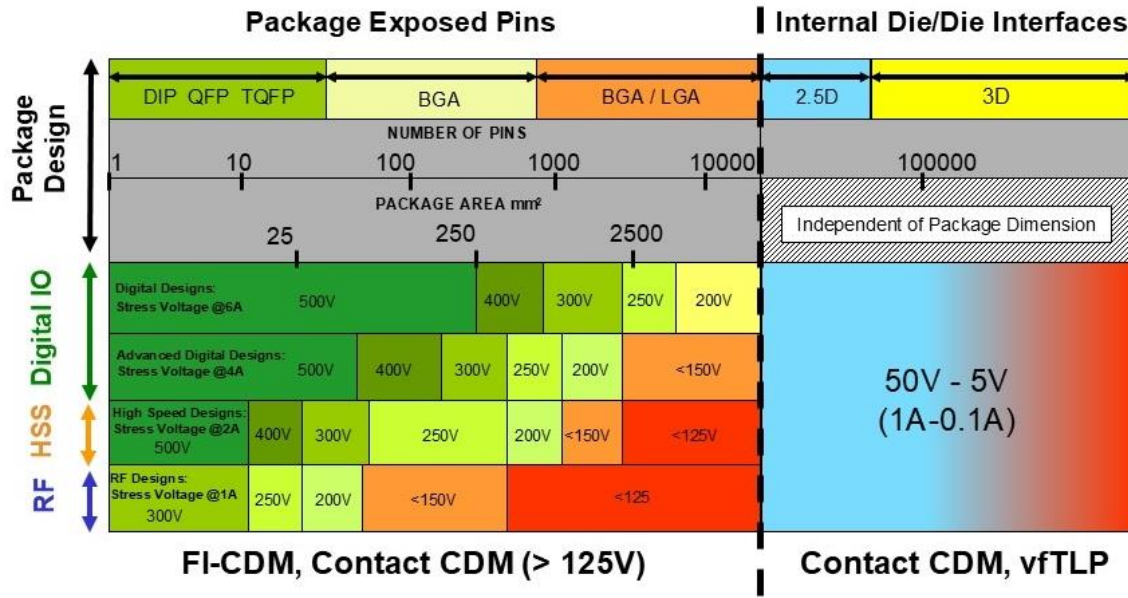
Figure 2: Combined Projected Effects of IO Design and IC Package Size on CDM
